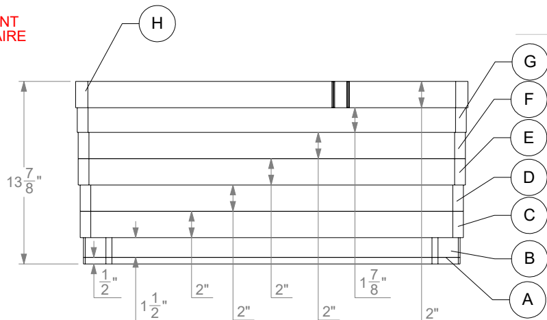
BASE TRAY - ELEVATION
